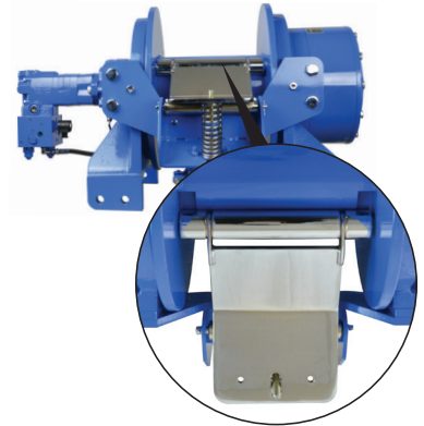
Superior cable-management Roller Tensioner
